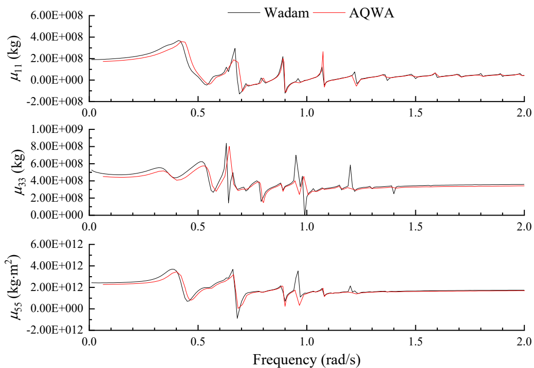
Figure 12 Added mass
